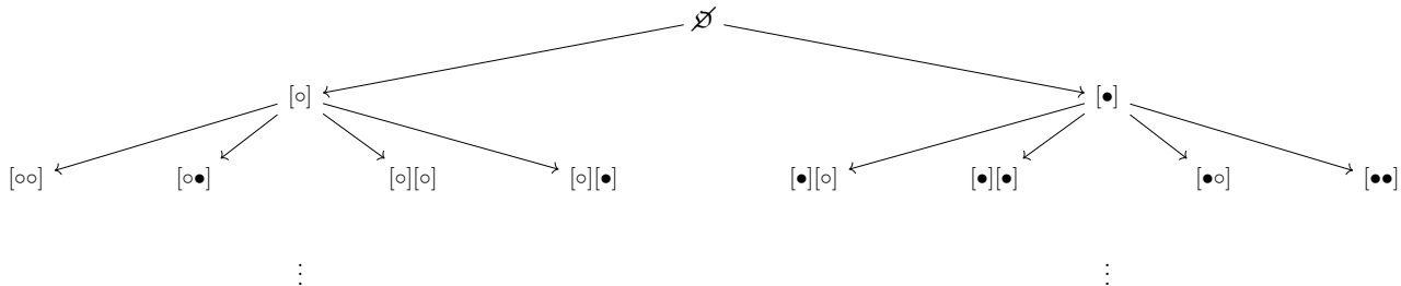
Figure 1: Constructing all 2-CCLOs of size 0, 1, 2
